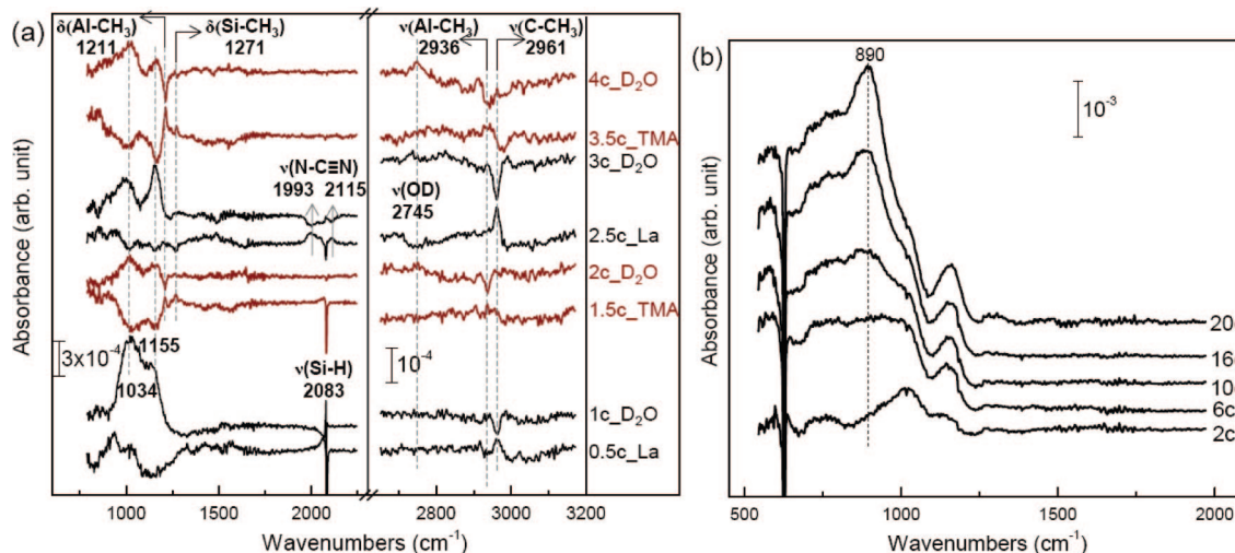
Figure 5. (a) Differential spectra of H/Si(111) upon exposure at 300 °C to \text{La}(\text{Pr-MeAMD})_3 (0.5c_La), \text{D}_2\text{O} (1c_ \text{D}_2\text{O} ) and trimethylaluminum (1.5c_TMA), \text{D}_2\text{O} (2c_ \text{D}_2\text{O} ) up to the fourth ALD cycle. Each spectrum is referenced back to the previously treated surface. (b) Absorbance spectra after 2, 6, 10, 16, or 20 cycles, referenced to the initial H/Si(111).
