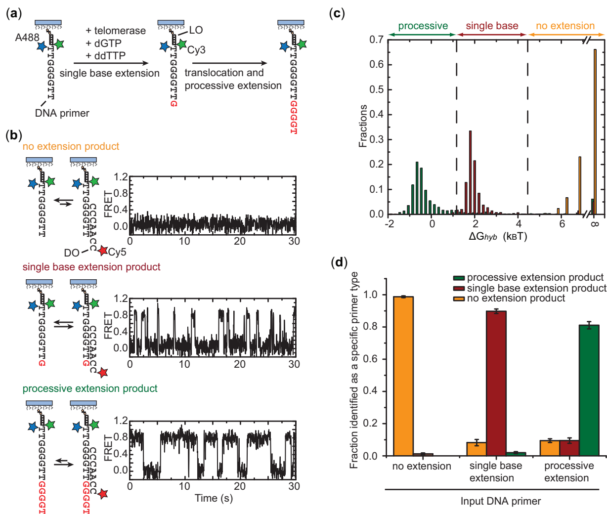
Figure 3. Single-molecule telomerase activity assay. (a) Schematics illustrating the three types of expected products from a telomerase-catalyzed primer extension reaction in the presence of dGTP and chain-terminating ddTTP. The Alexa Fluor-488 (A488, blue star) dye on the primer serves the purpose of primer density determination. Twenty nanomolar Cy3-labeled LO with a sequence complementary to the non-telomeric region of the primer is added to introduce the FRET donor Cy3 (green star) to the primer. (b) The three classes of primer-extension products show distinct hybridization kinetics with the Cy5-labeled DO, which is present at 300 nM in the imaging buffer. The hybridization kinetics were probed by FRET between the Cy3 (green star) on the primer and Cy5 (red star) on the DO. (c) The distribution of the hybridization free energy \Delta G_{hyb} derived from many primer molecules shows little overlap for standard primers representing the no extension (orange), single base extension (red) and processive extension (green) products of a telomerase reaction. The distribution for the no extension primers appears asymmetric because hybridizations between primer and DO that lasted shorter than one camera frame were indistinguishable and therefore were all binned as having a \Delta G_{hyb} equal to infinity. The vertical dashed lines represent the threshold values used to determine the length of an unknown primer. (d) Characterization of the error rates of the detection scheme using standard primers of known lengths: the orange, red and green bars indicate the fractions of primers identified as a no extension, single base extension and processive extension products. Error bars represent SD of the mean obtained from three independent experiments.
