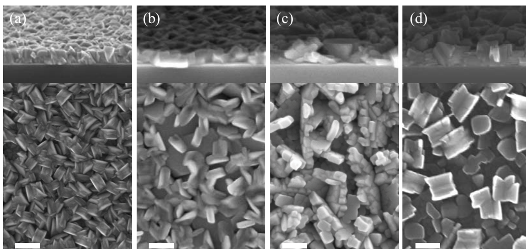
Figure 3. Plan-view and cross-sectional (12° tilt) SEM images of SnS films deposited on thermal oxide (SiO 2 ) for 1000 ALD cycles at (a) 120 °C, (b) 200 °C, (c) 250 °C, and (d) 300 °C. The scale bar is 200 nm.
