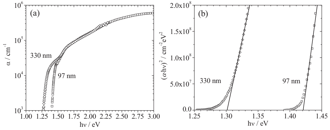
Figure 10. Optical properties of SnS films deposited at 200 °C at two different thicknesses. (a) absorption coefficient \alpha and (b) a plot of (\alpha \cdot h\nu)^2 as a function of photon energy, indicating direct transition with the optical band gap E_g at x-interception.
