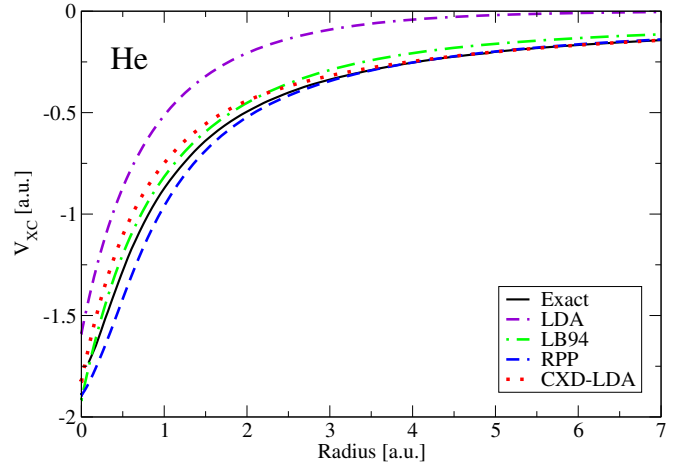
FIG. 8. CXD-LDA potential for helium. Comparison with the LDA, LB [11], RPP [20] and the exact [14] potentials.
