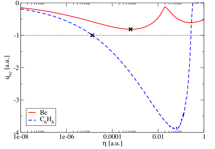
FIG. 5. The q_{xc}(\eta) function, Eq. (20), for LDA on atomic Beryllium atom and C_6H_6 . The crosses mark the position of \eta_0 , the optimal value of \eta .
