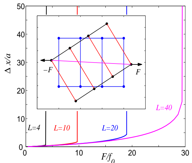
FIG. 6: Force vs. extension curves for the nonlinear vector generalization of the deGennes model with cross brace for L = 4, 10, 20, and 40 respectively. Inset is a configuration snapshot illustrating the rotation of the sheared DNA for L = 4 and a small force F = 0.093f_0 .
