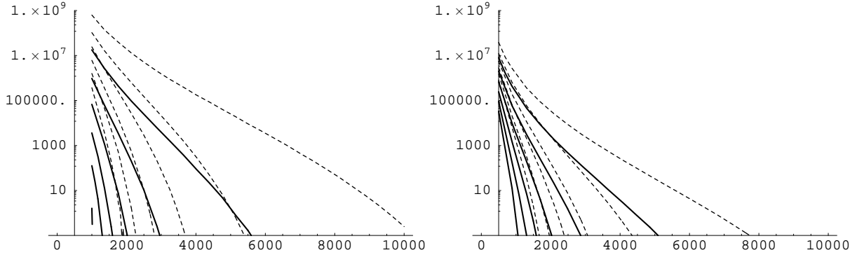
Figure 4: Total black hole cross section in femtobarns, including (solid curves) and not including (dashed) inelasticity as a function of M_D for ADD with n = 6 and \tilde{M} for RS1. The different curves from highest to lowest correspond to x_{min} = 1 - 6 .
