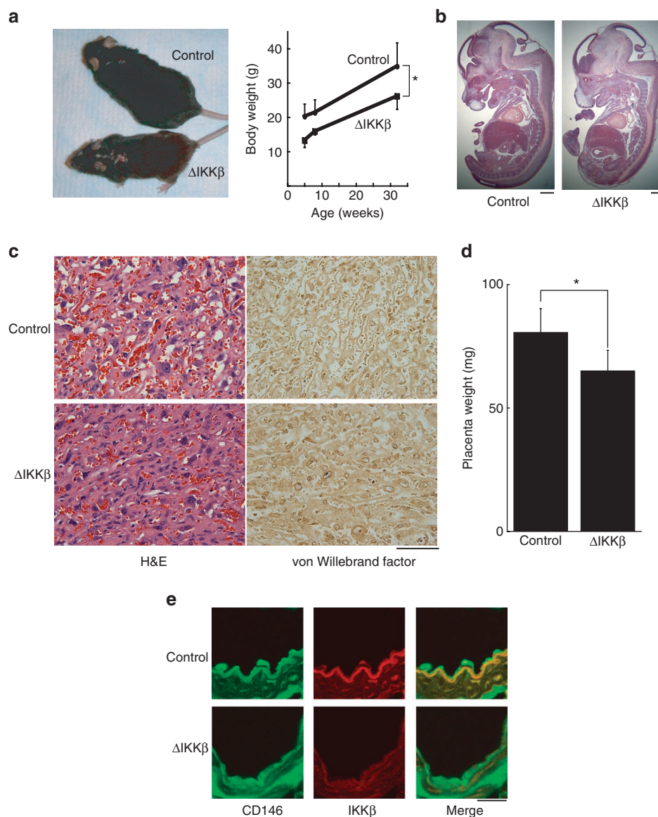
Figure 1 | Phenotype of endothelial-specific IKK \beta knockout mice. (a) Photograph of littermate wild type ('control') and IKK \beta^{\Delta\text{EC}} (' \Delta\text{IKK}\beta ') mice and body weight \pm s.d. shown from mice of each genotype at the indicated age ( n=3 /each group, *P < 0.005 in repeated two-way ANOVA). (b) H&E staining of embryos at E14. Scale bars: 1 mm. (c) Staining of placentae by H&E and immunohistochemistry for von Willebrand Factor at E14. Scale bars: 10 \mu\text{m} . (d) Placenta weight from mice of each genotype ( n=6 in IKK \beta^{\Delta\text{EC}} and n=3 in control mice, *P < 0.05 in two-sided Student's t -test. Error bars: \pm s.d.). (e) Confocal microscopy images of vascular endothelium in IKK \beta^{\Delta\text{EC}} and control mice immunostained with antibody for CD146 and IKK \beta . Scale bars: 100 \mu\text{m} .
