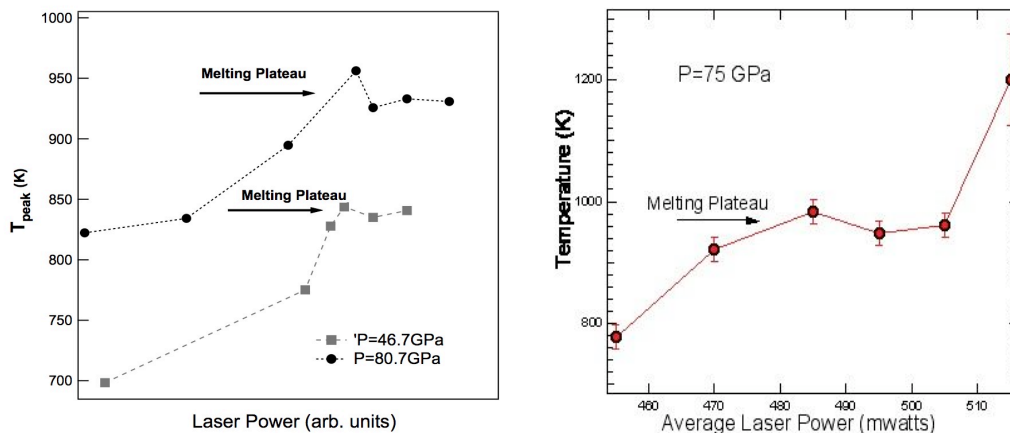
FIG. 9. Left: Plateaus at the melting line for hydrogen under high pressure.
