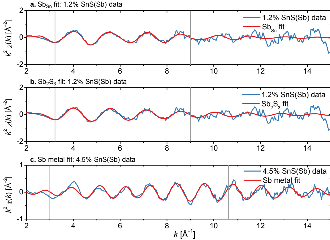
Figure 6. EXAFS data and fits for Sb edge: (a) 1.2% SnS(Sb) data with Sb Sn fit, (b) 1.2% SnS(Sb) data with Sb 2 S 3 fit, and (c) 4.5% SnS(Sb) data with Sb metal fit. The vertical lines denote the range chosen for Fourier transformation.
