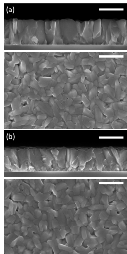
Figure 1. Cross-sectional and plan-viewed SEM images of (a) an undoped \text{SnS} film and (b) a \text{SnS}(5\% \text{ Sb}) film. The scale bar is 500 nm.
