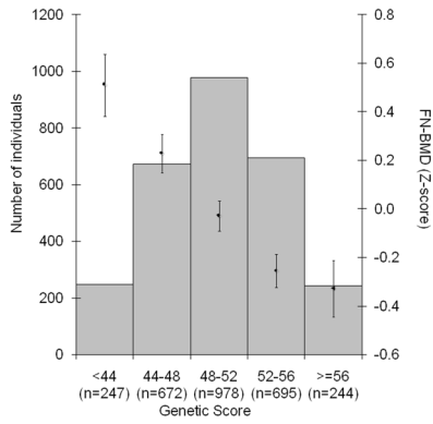
Figure 3. Combined effect of BMD-decreasing alleles and fracture risk-increasing risk alleles modelled in the population-based Prospective Epidemiological Risk Factor (PERF) study (n=2,836 women) on A) Baseline FN-BMD standardized residuals (Z-scores), B) Risk for Osteoporosis and C) Risk for Any type of fracture . The genetic score of each individual for A) and B) was based on the 63 SNPs displaying genome-wide significant association with BMD (55 main and 8 secondary signals), and for C) was based on the 16 BMD SNPs associated with fracture. Both genetic scores are weighted for relative effect sizes estimated without the PERF study. Weighted allele counts summed for each individual were divided by the mean effect size making them equivalent to the percent of alleles carried by each individual and binned into 5 categories. Histograms describe counts of individuals in each genetic score category (left axis scale). Diamonds (right axis scale) represent A) mean FN-BMD standardized levels, risk estimates in the form of odds ratio for B) Osteoporosis (defined as NHANES T-score<-2.5) and for C) Any type of Fracture using the middle category as reference (OR=1). Vertical lines represent 95% confidence limits.
