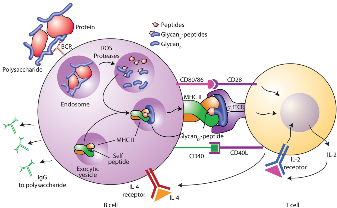
Figure 6. Mechanism of T-cell activation by glycoconjugate vaccines: a new working model
