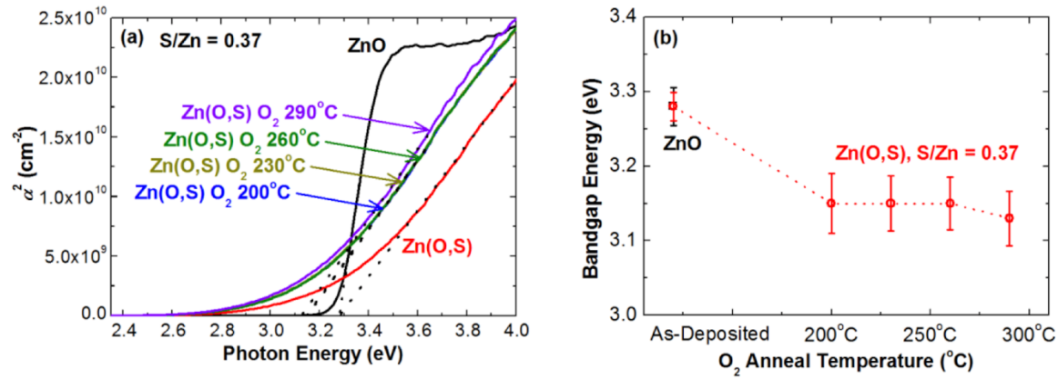
Fig. 3. Plots of (a) \alpha^2 vs. h\nu and (b) bandgap energy vs. O 2 annealing temperature for Zn(O,S) with S/Zn = 0.37.
