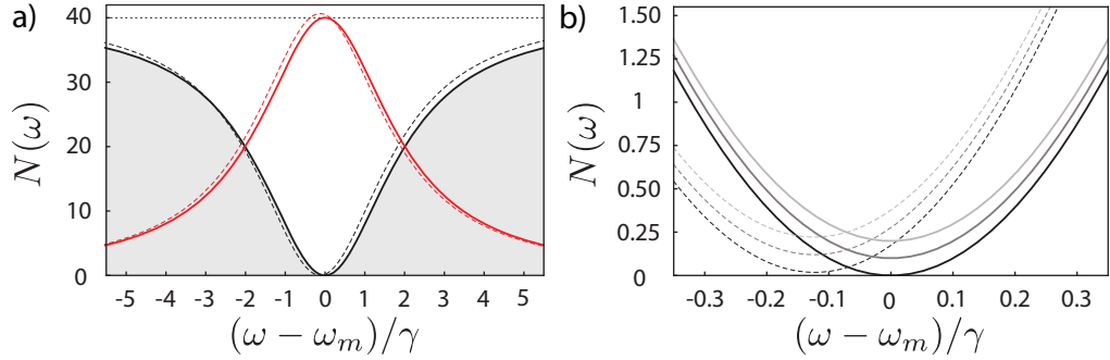
Figure 5. Detailed results for OM noise filtering. (a) Filtered phononic noise spectrum N_F(\omega) (black lines) and the corresponding photonic output spectrum (red lines), with the beam-splitter Hamiltonian (16) (solid lines) and with the full linearized Hamiltonian (15) (dashed lines). The parameters are \omega_m/\gamma = 1200 , \gamma_0 = 0 , \kappa/\gamma = 300 , g|\alpha| = \sqrt{(\gamma + \gamma_0)\kappa/2} and N_{\text{th}} = 40 . (b) Dip of the filtered noise spectrum N_F(\omega) for different values of the intrinsic mechanical damping rate \gamma_0/\gamma = 0, 0.0025, 0.005 .
