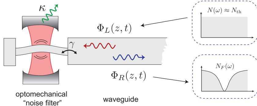
Figure 3. Setup for an OM noise filter (OM continuous mode cooling). A mechanical resonator is coupled to a continuous phonon waveguide ( \gamma ) and laser cooled via an optical cavity mode. Within a bandwidth \sim \gamma around the mechanical frequency, the incident thermal noise can be efficiently suppressed, creating a dip in the filtered noise spectrum N_F(\omega) of the reflected waveguide modes.
