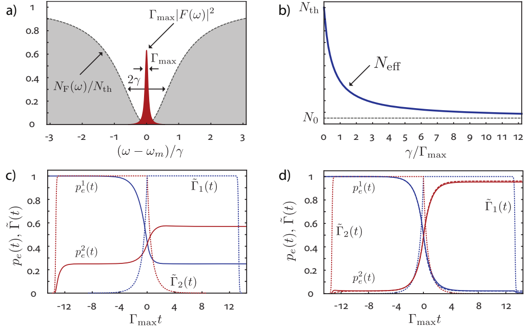
Figure 6. Quantum state transfer through a noisy channel. (a) Spectral overlap of the transfer pulse |F(\omega)|^2 and the filtered noise spectrum N_F(\omega) for N_0 = 0 and \Gamma_{max}/\gamma = 0.10 . (b) Effective occupation number N_{eff} as a function of \gamma/\Gamma_{max} for N_0/N_{th} = 0.05 . (c) Numerical simulation of a quantum state transfer in the presence of thermal noise with N_{th} = 0.5 . (d) The same state transfer with the OM noise filter switched on and \Gamma_{max}/\gamma = 0.10 . In both plots the blue and red solid lines show the excited state populations p_e^i(t) = \langle \sigma_+^i(t) \sigma_-^i(t) \rangle for qubits 1 and 2, respectively. The dotted lines show the corresponding pulse shapes \tilde{\Gamma}_i(t) = \Gamma_i(t)/\Gamma_{max} as defined in equation (51), but with cut-offs. In (d) the dashed line shows the results obtained from a two-qubit cascaded master equation with an effective thermal occupation number N_{eff} .
