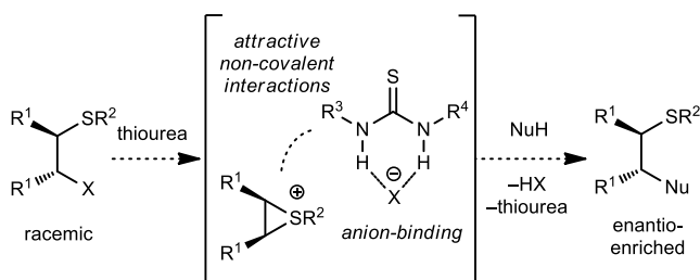
Figure 1. Proposed thiourea-catalysed episulfonium ion ring opening with indole via anion binding.
