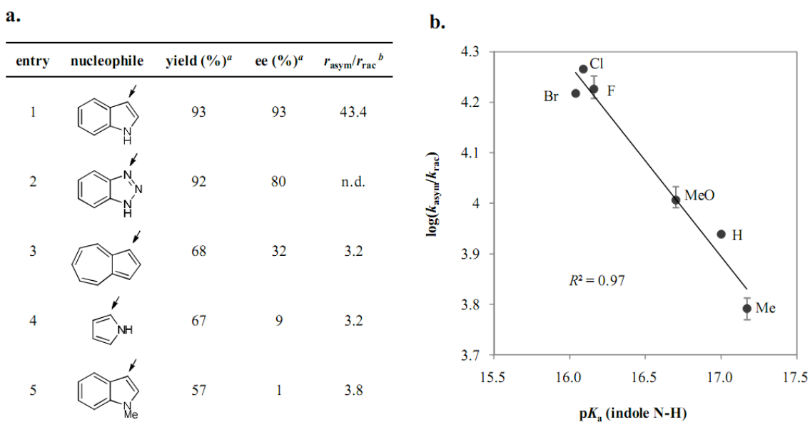
Figure 3. Reactivity- and enantioselectivity- dependence on the presence and the acidity of a N-H bond in the nucleophile. a. Structure-reactivity and -enantioselectivity relationship of \pi -nucleophiles. a Yields and enantiomeric excesses were obtained under reaction conditions described in eq. 2. b The initial reaction rates with 4-NBSA alone ( r_{\text{rac}} ) and with 4-NBSA/ 3e ( r_{\text{asym}} ) were determined directly by in situ IR spectroscopy. The ( r_{\text{asym}}/r_{\text{rac}} ) value was not determined for benzotriazole (entry 2) because the kinetic analysis was complicated by the poor solubility of the nucleophile in the reaction medium. b. Correlation between the degree of rate acceleration by 3e over the background racemic reaction ( k_{\text{asym}}/k_{\text{rac}} ) and the acidity of the N-H motif of 5-substituted indole derivatives ( \text{p}K_{\text{a}} ). The reaction rate constants ( k_{\text{rac}} and k_{\text{asym}} ) were determined by in situ IR and 1 H NMR spectroscopy (see Supplementary Information, Section 14 for detailed experimental procedure and data analysis). Error bars indicate the range of experimental data from 2-3 individual measurements, and the line represents least-squares fit.
