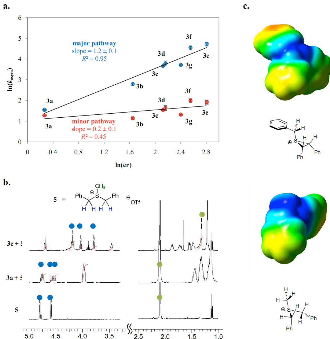
Figure 4. Enantioinduction is achieved by the thiourea catalysts through a selective, attractive cation- \pi interaction between the extended aromatic residue on the catalyst and the acidic \alpha -protons in the episulfonium ion. a. Correlation between rate and enantioselectivity of reactions catalysed by thioureas 3a-3g . Each data point represents the average rate determined from two individual kinetic experiments, with the error bar showing the range of the measurements. The rate constants for the major and the minor pathways ( k_{\text{asym,major}} and k_{\text{asym,minor}} , respectively) are calculated on the basis of the rate equations (eqs. 3 & 4) and the following equations: (a) r_{\text{asym}} = r_{\text{asym,major}} + r_{\text{asym,minor}} (b) er = r_{\text{asym,major}}/r_{\text{asym,minor}} . Lines represent least-squares fits. b. ^1\text{H} NMR binding study of thiourea and 5 in d_8 -toluene, showing attractive interactions between the aromatic group in 3e and the \alpha -protons in 5 . The resonances of the benzylic protons and the methyl protons in 5 are labeled with blue and green dots, respectively. In the two bottom spectra, the methyl resonance overlaps with the solvent peak, but can be identified when zoomed-in. c. Electrostatic potential maps for fully optimized structures (B3LYP/6-31G(d)) of the episulfonium ion derived from 1a and the sulfonium ion in 5 , revealing a similar distribution of positive charge over the benzylic protons. Negative potentials are shown in red and positive potentials in blue.
