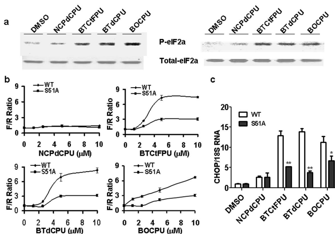
Figure 2. N,N' -diaryllureas reduce the abundance of the ternary complex by causing phosphorylation of eIF2α
