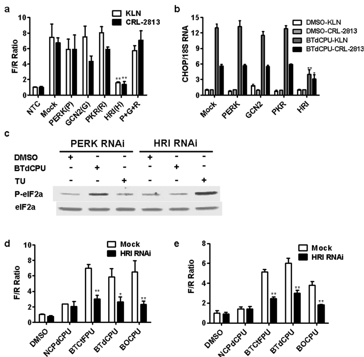
Figure 3. The N,N' -diarylureas specifically activate HRI kinase
