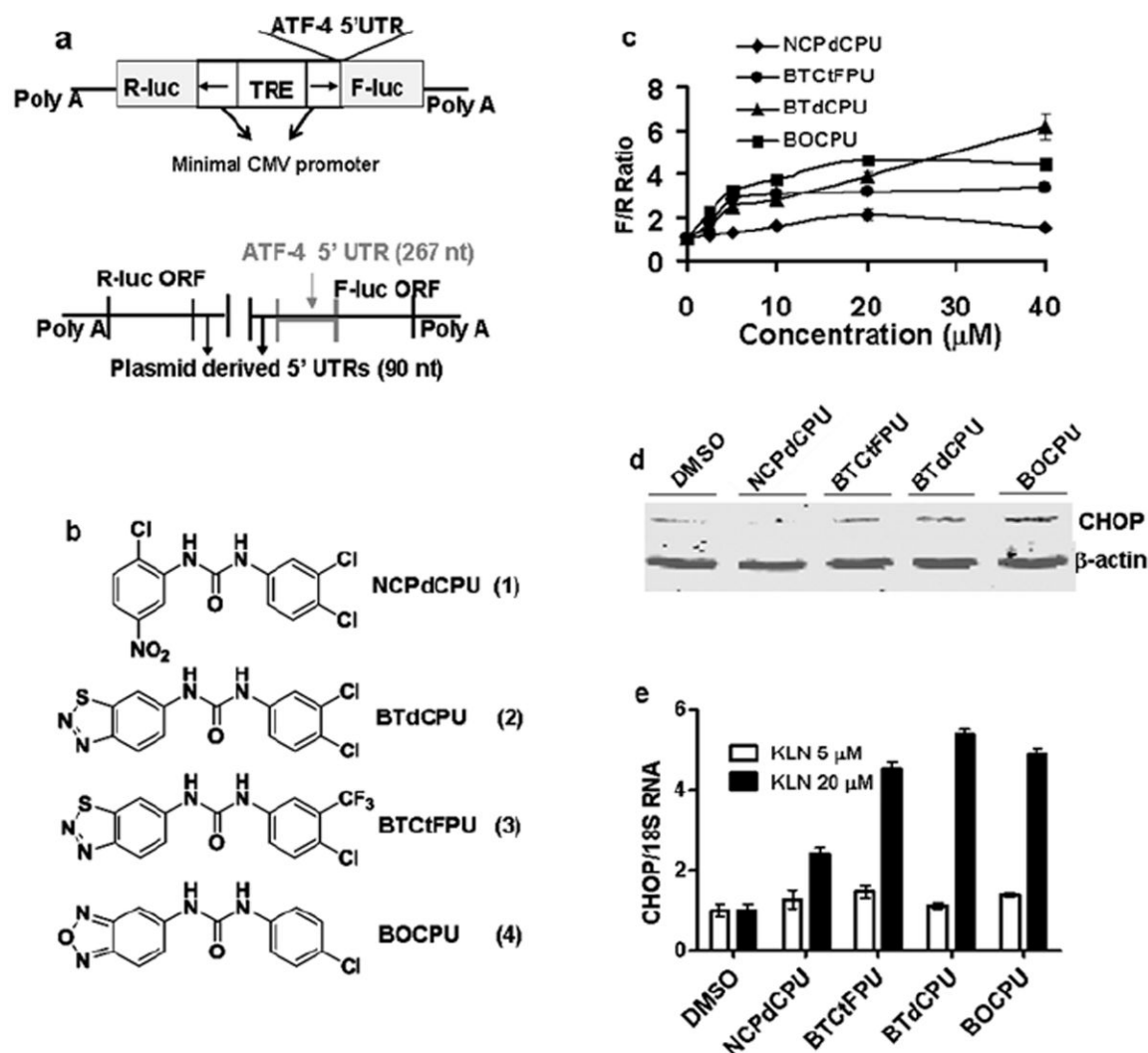
Figure 1. Identification and validation of the N,N' -diarylsureas as modifiers of the ternary complex abundance
