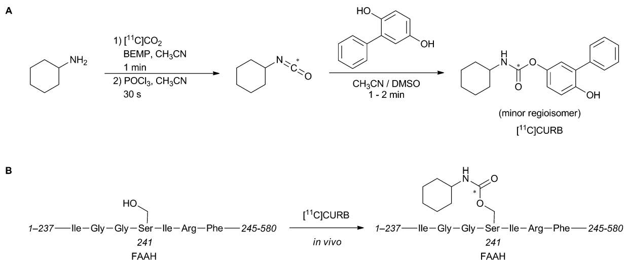
Scheme 5 (A) Radiosynthesis of [ ^{11}\text{C} ]CURB; (B) To effectively measure brain levels of FAAH using [ ^{11}\text{C} ]CURB, the radiolabel must be located on the carbonyl or N -alkyl fragment of the tracer. Asterisk denotes ^{11}\text{C} .
