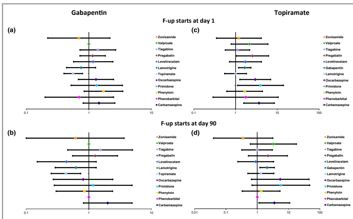
Figure 5. HdPS-matched rate ratios of ischemic coronary or cerebrovascular events a comparing initiators of single anticonvulsant agents against new users of gabapentin or topiramate. b a Myocardial infarction, acute coronary syndrome, cardiac revascularization procedure, death for ischemic heart disease, ischemic cerebrovascular events, ischemic stroke, or ischemic cerebrovascular death. b AT, as-treated analysis censoring at termination of exposure risk window, switching to another anticonvulsant agent, occurrence of a study event, death from causes not included in the study outcome, end of continuous health plan enrollment, or the end of the study period, whichever came first. hdPS indicates high-dimensional propensity score; ACs, anticonvulsants.
