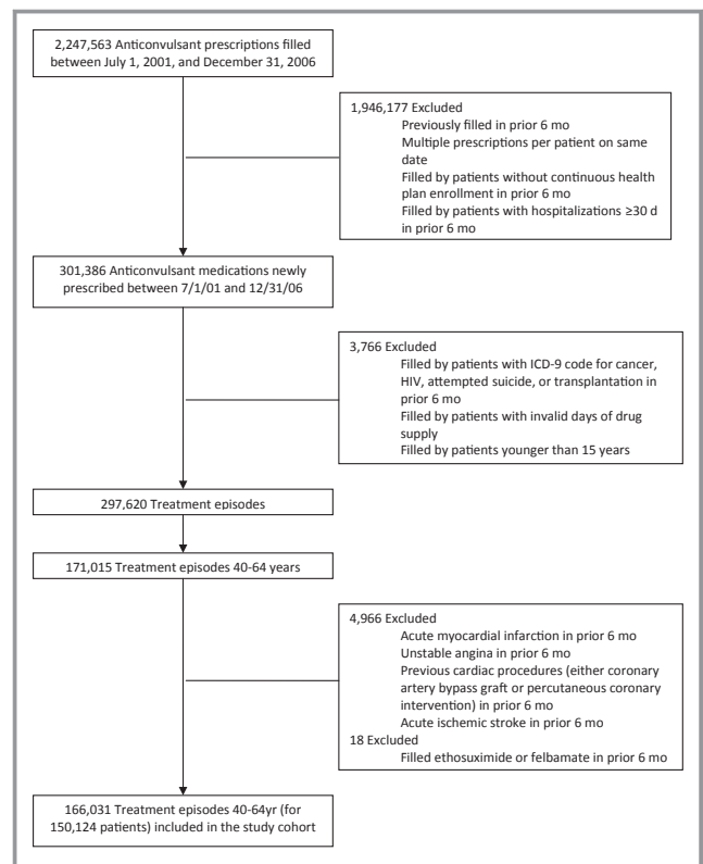
Figure 1. Flowchart of study cohort.
