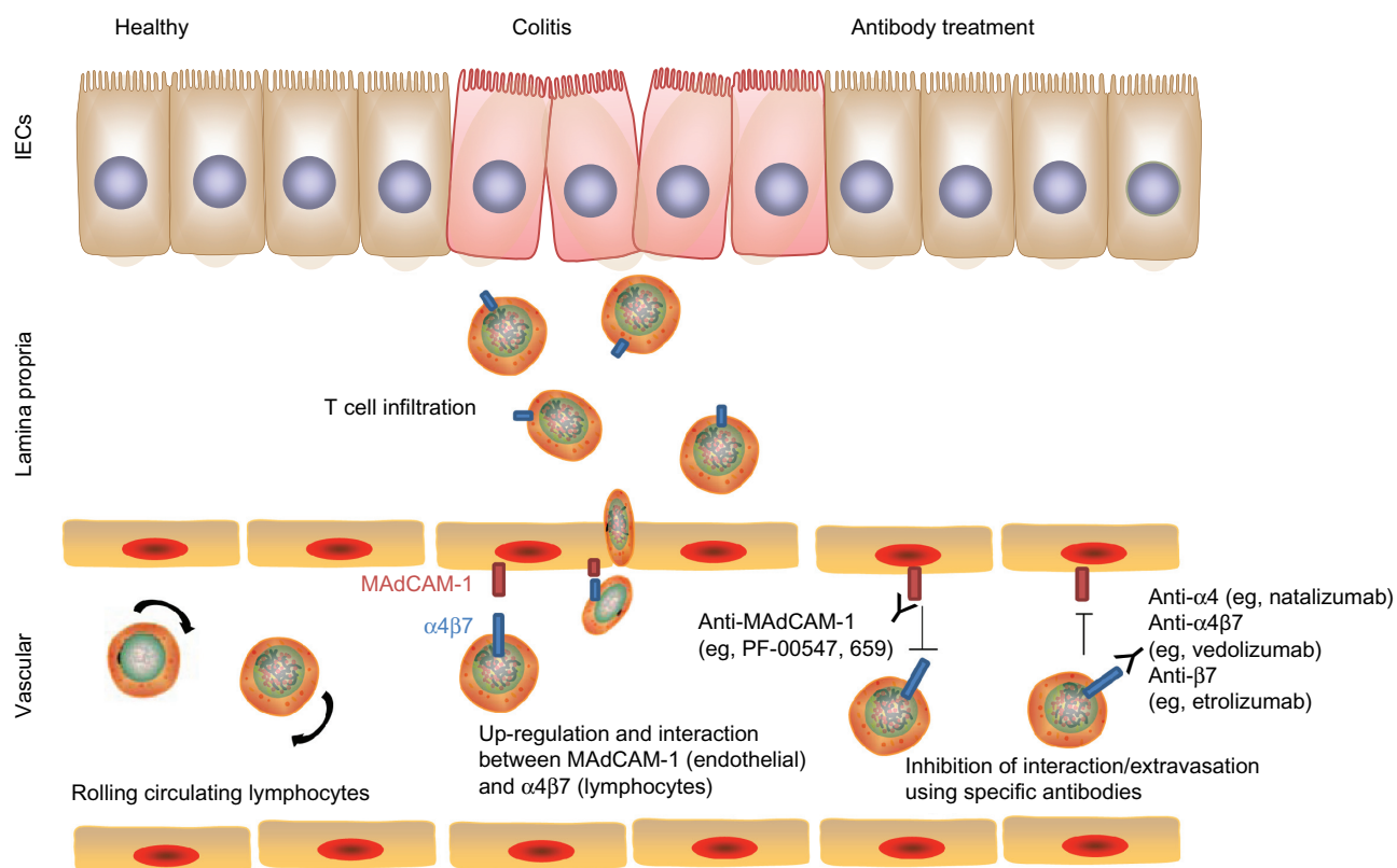
Figure 5 Blocking of immune cell trafficking to the colon. Upregulation of mucosal addressin cell adhesion molecule-I (MAdCAM-I) on intestinal vascular cells and expression of integrins (eg, \alpha 4\beta 7 ) on lymphocytes promote interaction and adhesion of lymphocytes onto the intestinal endothelium and subsequent extravasation into colonic tissues. Blocking MAdCAM-I or \alpha 4\beta 7 using specific antibodies disrupts this interaction and control of colitis severity.
