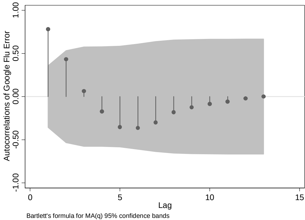
Fig 5. Autocorrelation plot for GFT post-update errors, post-September 22, 2013. A correlogram (graph of autocorrelations) of GFT errors since the latest update. 95% confidence intervals (shaded region) based on Bartlett's formula for MA(q) processes. Even for this short time period (30 weeks) the test for an AR(1) process rejects the null hypothesis of no autocorrelation at the 95% level.
