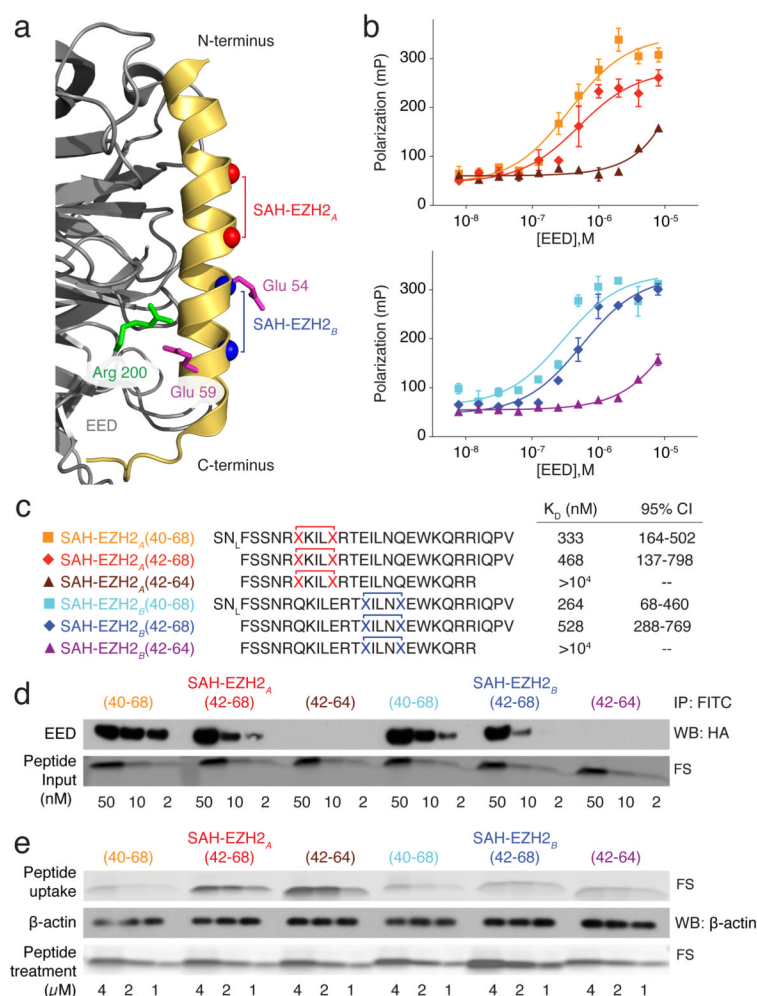
Figure 1. Synthesis, EED-binding activity, and cellular penetration of SAH-EZH2 peptides
