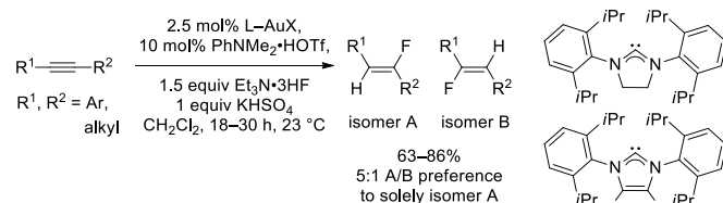
Scheme 133. Au-catalyzed hydrofluorination of alkynes
