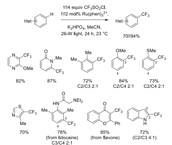
Scheme 59. Ru-photoredox-catalyzed trifluoromethylation of arenes and heteroarenes
