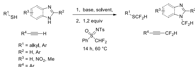
Scheme 51. Difluoromethylation S -, C -, N -nucleophiles with N -tosyl- S -difluoromethyl- S -phenylsulfoximine
