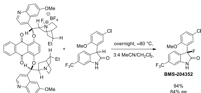
Scheme 14. Enantioselective α-fluorination of oxindoles mediated by N-fluoroammonium salts of cinchona alkaloids
