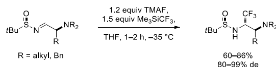
Scheme 88. Diastereoselective addition of \text{TMSCF}_3 to N -( tert -butylsulfinyl)imines
