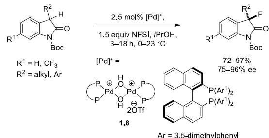
Scheme 12. Pd-catalyzed asymmetric \alpha -fluorination of oxindoles.
