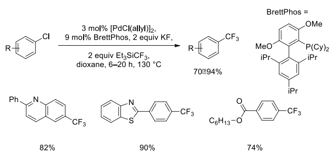
Scheme 85. Pd-catalyzed cross-coupling of aryl halides with \text{TMSCF}_3
