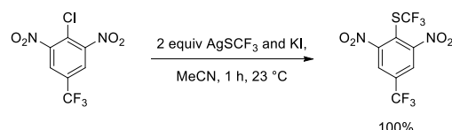
Scheme 117. Nucleophilic aromatic substitution with silver trifluoromethylthiolate
