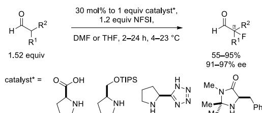
Scheme 16. Organocatalytic asymmetric α-fluorination of α-branched aldehydes
