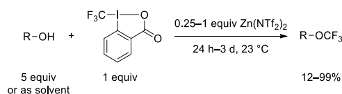
Scheme 110. O-Trifluoromethylation of alcohols with Togni reagent II
