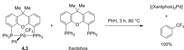
Scheme 84. Reductive elimination of trifluoromethyl arenes from \text{Pd(II)} complex
