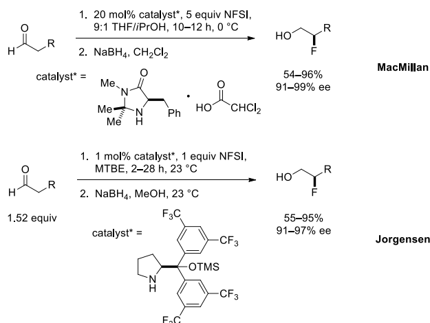
Scheme 15. Organocatalytic asymmetric α-fluorination of aldehydes
