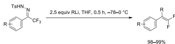
Scheme 141. Alkyl lithium-induced rearrangement of aryl trifluoromethyl tosylhydrazones to terminal 1,1-difluorostyrenes
