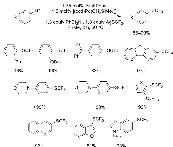
Scheme 121. Pd-catalyzed cross-coupling of aryl bromides with silver trifluoromethylthiolate activated with tetrasubstituted ammonium iodide
