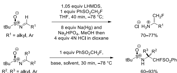
Scheme 42. Monofluoromethyl pronucleophile addition to chiral N -( tert -butylsulfinyl)aldimines and ketimines
