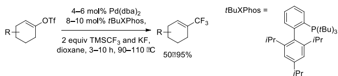
Scheme 86. Pd-catalyzed trifluoromethylation of alkenyl triflates
