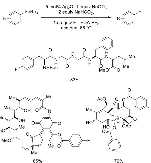
Scheme 6. Ag-catalyzed fluorination of complex aryl stannanes
