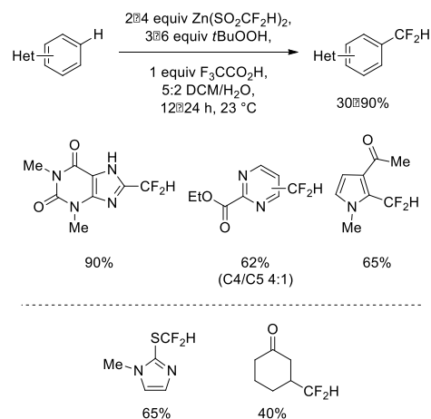
Scheme 47. Radical difluoromethylation of heteroarenes with Zn(SO 2 CF 2 H) 2 and tert -butylhydrogen peroxide
