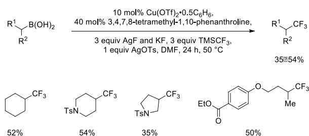
Scheme 75. Cu-promoted oxidative trifluoromethylation of secondary alkylboronic acids
