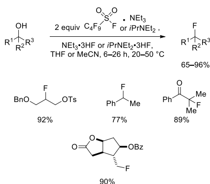
Scheme 35. Deoxyfluorination of various alcohols with perfluorobutanesulfonyl fluoride-trialkylamine adduct and TREAT·HF
