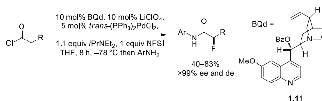
Scheme 17. Organocatalytic asymmetric α-fluorination of acid chlorides
