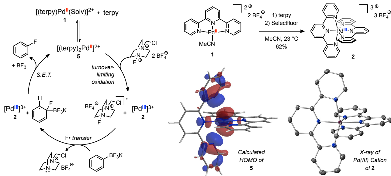
Scheme 2. Proposed Mechanism for Pd-Catalyzed Fluorination, Synthesis and X-ray Structure of Pd(III) Intermediate 2, and DFT Calculated Structure of Pd(II) Intermediate 5 a
