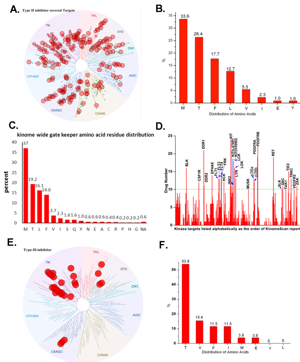
Figure 7. Analysis of selectivity profiling revealed type II binding kinases. (A) Treespot demonstration of kinase distribution among kinome. (B) Analysis of gatekeeper residues among the type II inhibitor targeted kinases. (C) Analysis of gatekeeper residues among the kinome. (D) Statistics of most targeted kinases by type II inhibitors. (E) Treespot demonstration of most targeted kinase distribution among kinome. (F) Analysis of gatekeeper residues of most targeted kinases by type II inhibitors.
