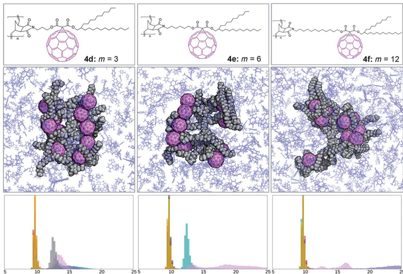
Fig. 2 (Top) Structural formula of the model molecules studied in the MD simulation, with different spaces (CH 2 ) m between the poly(norbornene) backbones and the C 60 units. (Middle) The snapshots of structures with m = 3 , m = 6 , and m = 12 after 20 ns of MD simulations in an explicit toluene solvent. (Bottom) The histogram of the distances between adjacent C 60 units, calculated based on the centers of mass of each fullerene. Distances (in Å) between each pair of C 60 units are shown in a unique color (see ESI† for the color code).
