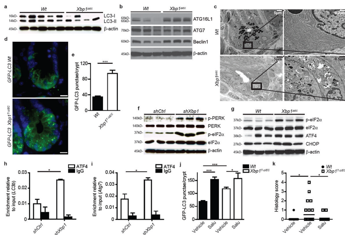
Figure 1. PERK/eIF2α signaling induces autophagy in Xbp1 -deficient intestinal epithelial cells a, b , Immunoblot for LC3 conversion in isolated primary IECs ( a ) ( n=5/4 ) and for autophagy proteins in primary IEC scrapings ( b ) ( n=3 ). c , Transmission electron microscopy (TEM) of crypts. Note autophagic vacuoles in various stages of evolution in Xbp1 ΔIEC hypomorphic Paneth cells. d, e , Crypt showing GFP-LC3 punctae ( d ), quantified in ( e ) ( n=10 ; unpaired Student's t-test). Bar, 5 μm. f, g , Immunoblot of silenced MODE-K cells ( f ) and primary IEC scrapings ( g ) for the PERK/eIF2α branch ( n=3 ). h, i , Promoter sequence qPCR for Map1lc3b ( LC3b ) ( h ) and Atg7 ( i ) after anti-ATF4 ChIP (unpaired Student's t-test). j , GFP-LC3 punctae per crypt after treatment with tamoxifen for 3 days and vehicle or salubrinal ( n=10 ; one-way ANOVA with post-hoc Bonferroni). k , Enteritis histology score after salubrinal and tamoxifen co-treatment ( n=12/14/13 ; median shown; Kruskal-Wallis with post-hoc Holm's-corrected Mann-Whitney U). Results represent three ( a, f, g ) or two ( c, e, h, i ) independent experiments. * P < 0.05 , *** P < 0.001 .
