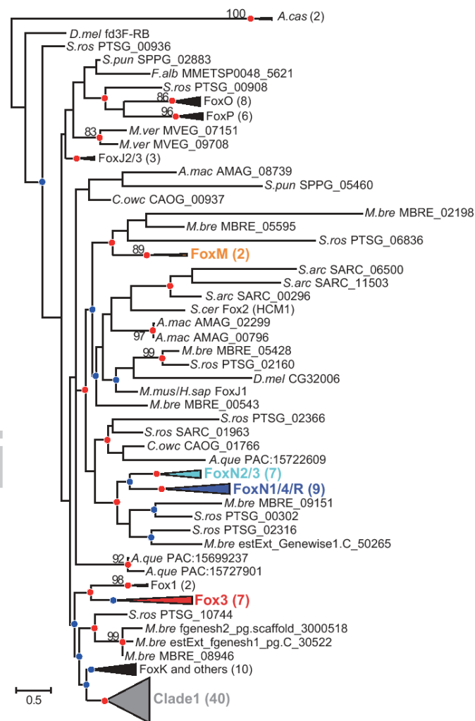
Fig. 2. Maximum likelihood phylogenetic tree of forkhead domains. This compact tree was constructed for presentation purposes from a representative subset of phylogenetically informative species: metazoans mouse, fly and sponge; choanoflagellates Salpingoeca rosetta and Monosiga brevicollis ; Capsaspora owczarzaki and Sphaeroforma arctica from Ichthyosporae; Saccharomyces cerevisiae from Dikarya; Allomyces macrogynus from Blastocladiomycota; Spizellomyces punctatus from Chytridiomycota; Mortierella verticillata from Mortierellomycotina; Fonticula alba from Nucleariida; Acanthamoeba castellanii from Amoebozoa. Nodes supported with strong likelihood ratios are indicated with red circles (aLRT \geq 99\% ) or blue circles (aLRT \geq 95\% ); bootstrap support values are shown for nodes with \geq 80\% support. Clades containing alternate binding specificities are highlighted in color (see text). Importantly, the groupings of subfamilies in this tree and the complete tree with all Fox domains are almost identical to each other (see Figure S2).
