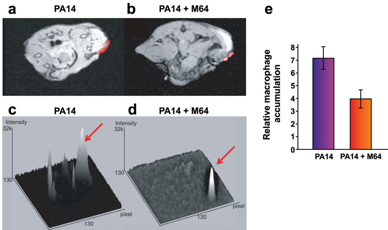
Figure 8. Magnetic resonance imaging of M64 inhibition of macrophage recruitment at a burn and infection site. a–e. In vivo positive contrast imaging of mice infected with PA14, plus and minus M64. The off resonance imaging transverse relaxation in the rotating frame (ORI-T2 \rho ) images were transformed to signal to noise ratio (SNR) images and thresholded in units of image standard deviation. a., b. The positive-contrast images are presented in pseudocolor, thresholded to signal greater than three in dimensionless SNR units, and superimposed on a FLASH image. For image processing, regions of interest (ROI) were drawn around the burn region and the total thresholded signal intensity was integrated within each ROI. Similar slices were chosen at the same anatomical location in all mice. c., d. 3-dimensional graphs of pixel intensities show an intense peak in the burn area for the PA14 control mouse, with this peak reduced by M64. e. Signal was measured in units of SNR, thresholded at three standard deviations, and measured within ROIs at the level of the burn and infection. The noise threshold was estimated by fitting the image background to a Rician distribution. Error bars depict standard error of the mean image intensity in the ROI. Error bars depict mean \pm SD of at least 3 replicates. Difference between PA14 and PA14 + M64 is statistically significant ( p < 0.05 , unpaired t test). doi:10.1371/journal.ppat.1004321.g008
