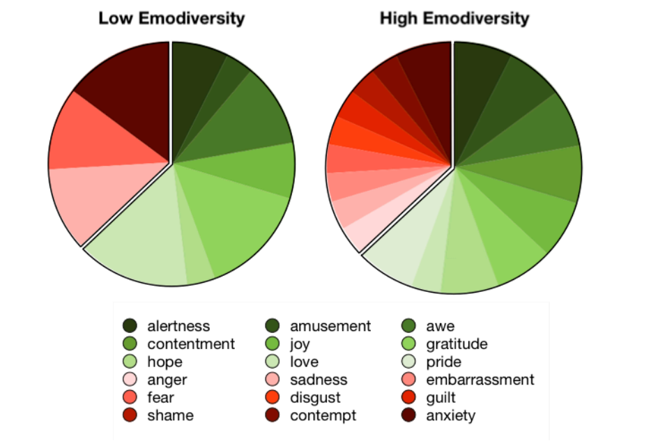
Figure 1. Schematic representing prototypical respondents low and high in global emodiversity, respectively. Selected respondents have identical mean levels of positive (green) and negative (red) emotion – matching the sample means (Positive Emotion = 1.89; Negative Emotion = 1.11) – but varied widely in emodiversity.
