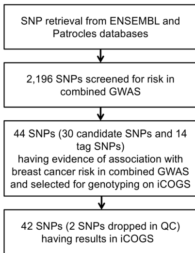
Figure 1. Workflow of miRNA SNP selection. doi:10.1371/journal.pone.0109973.g001
