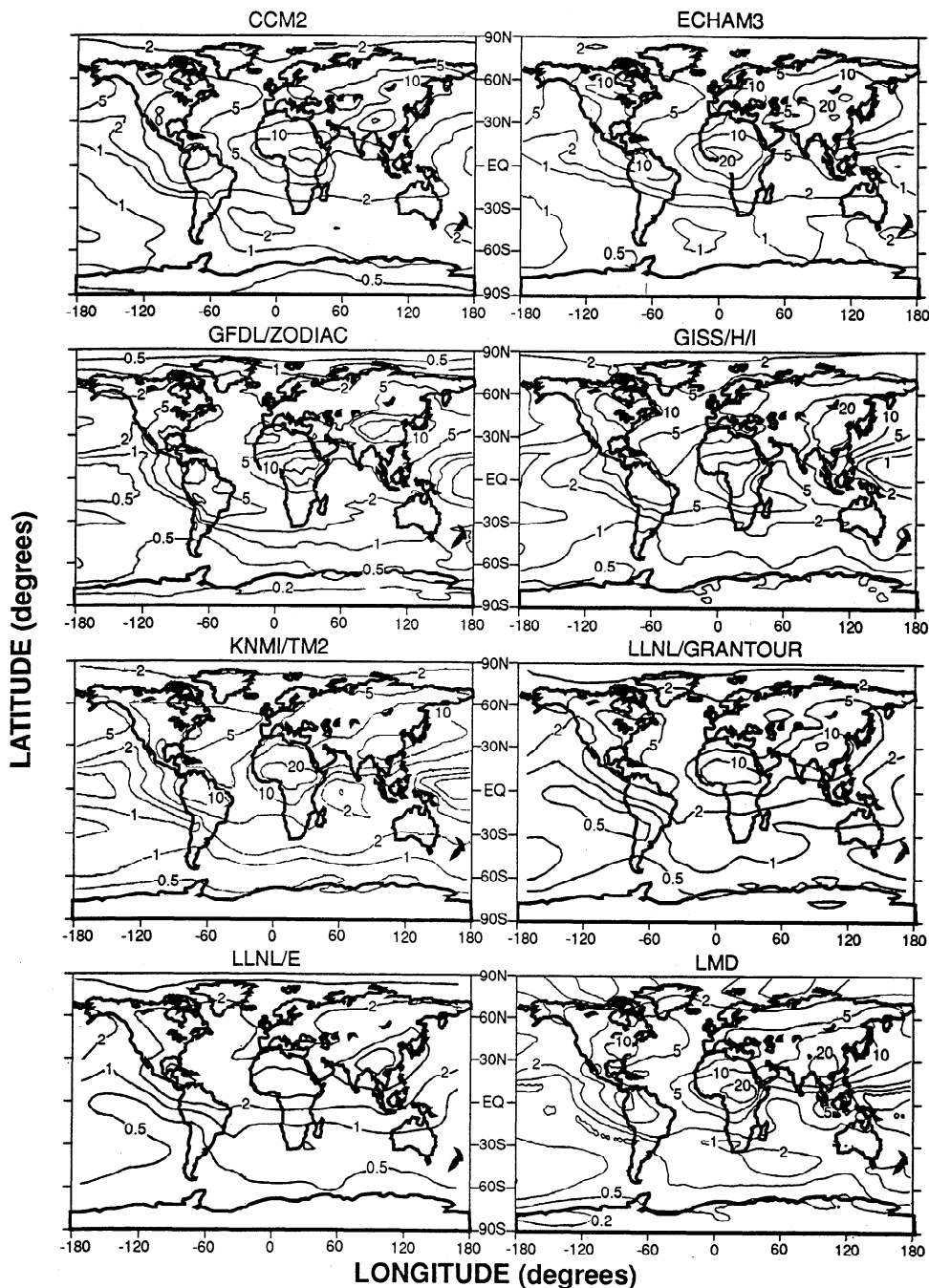
Figure 4. Mean 222 Rn concentrations simulated by the different models at 300 hPa in June-August. Units are 1 \times 10^{-21} mol/mol; see text for conversion factors.
