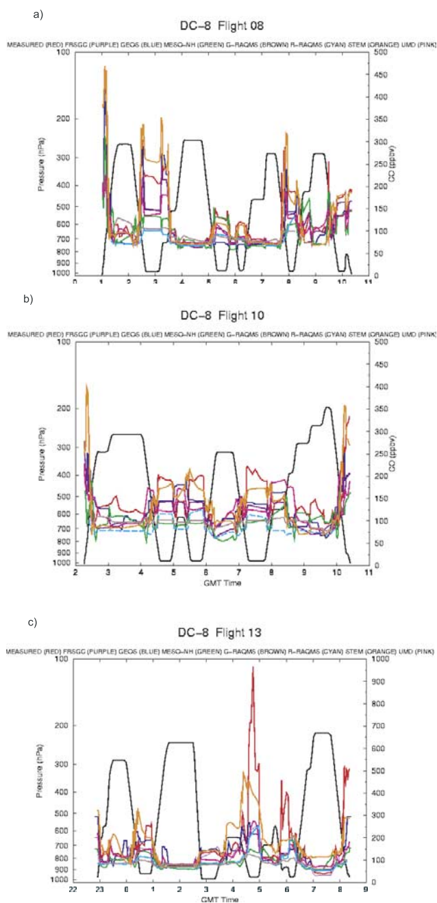
Figure 3. Time series of aircraft altitude (black), aircraft-derived CO (red), and the seven model-derived simulations for (a) DC-8 flight 8, (b) DC-8 flight 10, and (c) DC-8 flight 13. FRSGG/UCI (violet), GEOS-CHEM (blue), Meso-NH (green), RAQMS Global (brown), RAQMS Regional (cyan), STEM (orange), UMD CTM (pink).
