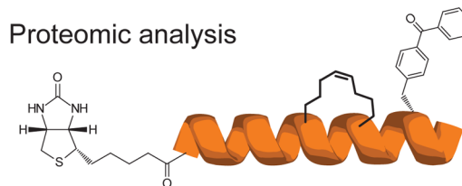
Figure 5. Design and derivatization of stapled peptides for a diversity of research applications. We have generated stapled peptides for (1) cellular studies by optimizing \alpha -helicity and adjusting overall charge to the 0 to +2 range, (2) PRE NMR analyses by optimizing solubility with overall negative charge and appending differentially localized spin labels, (3) fluorescence polarization binding and cellular uptake analyses by N-terminal derivatization with FITC, (4) in vivo PK and extracellular targeting studies of lengthy \alpha -helices by inserting two staples, (5) protein interaction discovery and helix binding site identification by inserting photoreactive non-natural amino acids along the length of an N-terminally biotinylated stapled peptide followed by affinity capture and mass spectrometry analysis.
