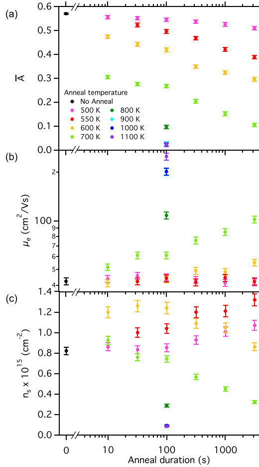
FIG. 3. Evolution of the optical and electrical properties with annealing duration and temperature. (a) Average sub-band gap absorbance from 1200–2300 nm. ((b) and (c)) Electron mobility and sheet carrier concentration, respectively, for each of the samples in (a). In all panels, the black data points indicate the corresponding measurements on the un-annealed sample (anneal duration of zero).
