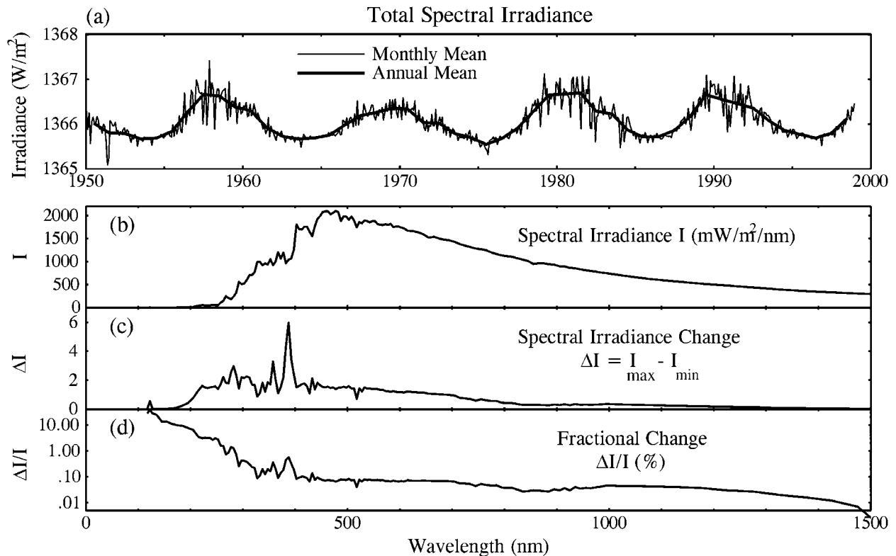
Figure 4. Solar irradiance characteristics based on data from analysis of J. Lean (1999): (a) total irradiance for the period 1950–1998, (b) spectral variation of irradiance, (c) spectral irradiance change between solar minimum (1996) and solar maximum (1989), and (d) the fractional irradiance change between solar maximum and solar minimum.
