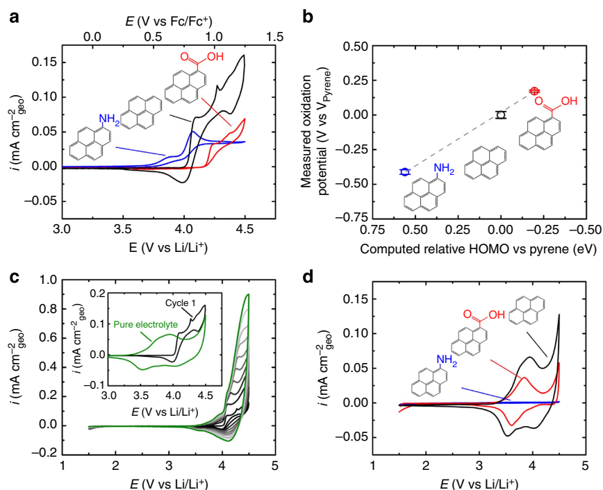
Figure 2 | Electrochemical polymerization reaction of pyrene derivatives on a GCE. (a) The first CV scan at 1 mV s -1 of 1 mM aminopyrene (blue), pyrene (black) and pyrenecarboxylic acid (red) molecules in solution of EC:DMC (3:7 volume ratio) with 1 M \text{LiPF}_6 . (b) Measured change in oxidation onset potential of 1 mM of aminopyrene (blue), pyrene (black) and pyrenecarboxylic acid (red) molecules in solution from pyrene during CV at 1 mV s -1 as a function of the computed relative HOMO energy level to that of pyrene. Grey line indicates the linear fit between calculated and experimental values. (c) Cyclic voltammogram of polymerization reaction and growth of lower potential redox reaction during 10 cycles at 1 mV s -1 in 1 mM pyrene. (Inset) Overlap of initial polymerization cyclic voltammogram of pyrene and subsequent cyclic voltammogram of polymerized pyrene in pure electrolyte of 1 M \text{LiPF}_6 in EC:DMC (3:7 volume ratio). (d) Cyclic voltammogram of polymerized aminopyrene (blue), pyrene (black) and pyrenecarboxylic acid (red) film during CV at 1 mV s -1 in 1 M \text{LiPF}_6 in a mixture of EC and DMC (3:7 volume ratio).
