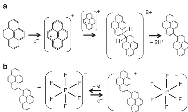
Figure 3 | Proposed polymerization and reversible redox reactions.
