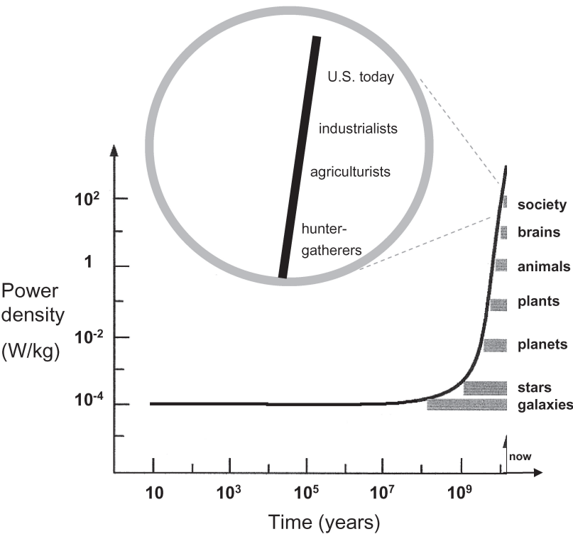
Fig. 1. Temporal dependence of energy rate density for a wide spectrum of energy-using systems over billions of years, including (within the circle, which magnifies part of the curve at top right) per capita power usage during the cultural advancement of human society in much more recent times. Adapted from Chaisson [2003].
