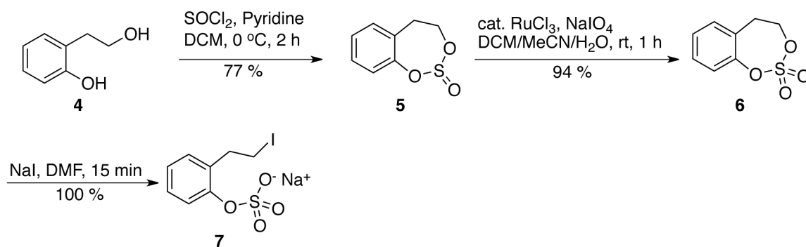
Scheme 1. Synthesis and Ring opening of Cyclic Sulfate 6
