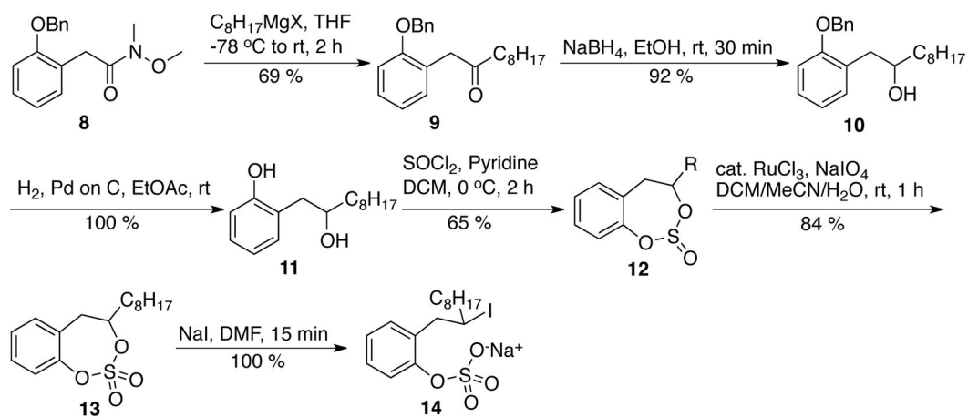
Scheme 2. Synthesis and Ring opening of Cyclic Sulfate 13
