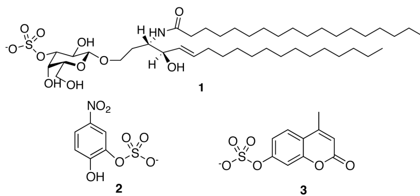
Figure 1. Natural and known phenolic substrates of ARSA.
