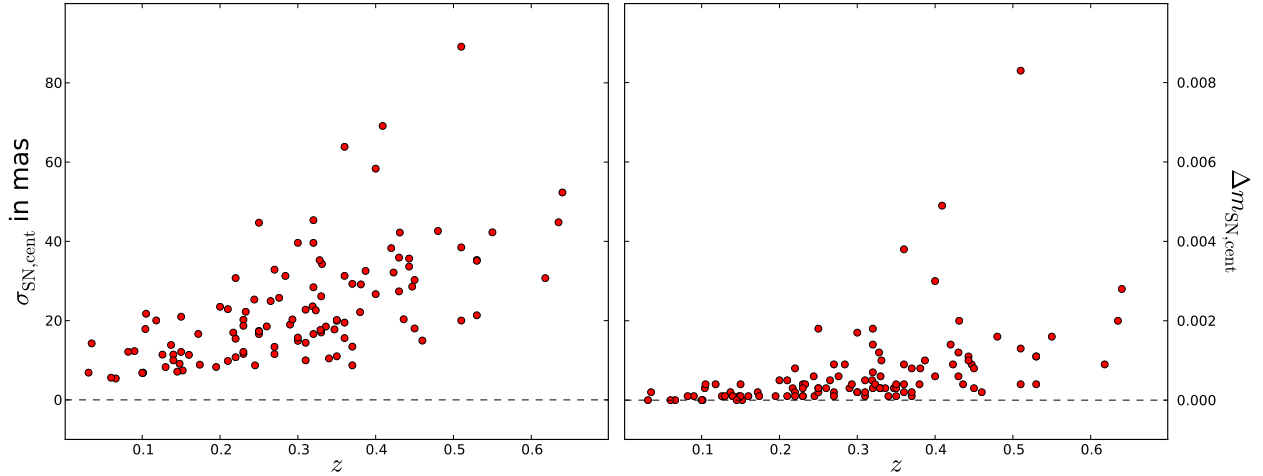
Figure D3. Left: The astrometric uncertainty in the SN centroid position determined by averaging the position of all detections versus redshift. The uncertainty in the SN centroid increases with increasing redshift. Right: The expectation value of the photometric bias due to the centroid uncertainty calculated with Equation D5.
