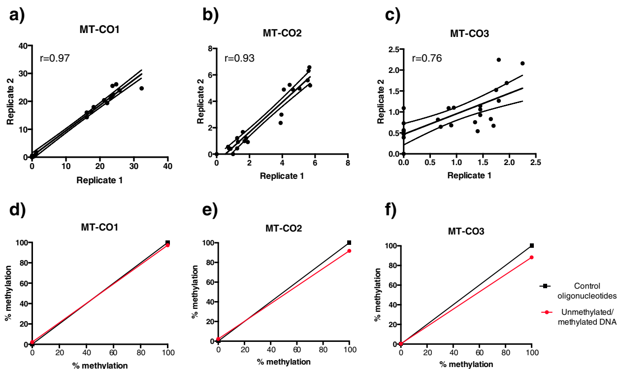
Figure 4 Technical replicates and quantitative validation of mtDNA pyrosequencing assays. Spearman correlation coefficients ( r ) of the technical replicates (replicates 1 and 2) for the designed pyrosequencing assays were (a) 0.97 for MT-CO1 , (b) 0.93 for MT-CO2 , and (c) 0.76 for MT-CO3 . The plot curve is displayed with a 95% confidence band. The quantitative validation of 0% and 100% methylated DNA for the (d) MT-CO1 , (e) MT-CO2 , and (f) MT-CO3 assays (red circle) were compared with 0% and 100% control oligonucleotides (black rectangle).
