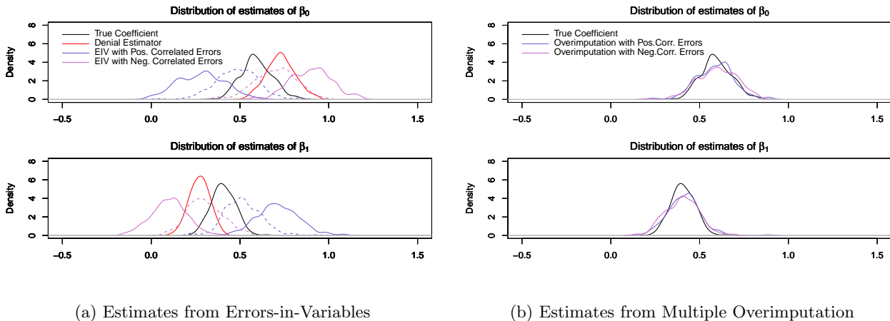
Figure 5: With data generated so that proxy variables are correlated with the dependent variable, EIV (left graphs) gives biased estimates whereas MO (right graphs) gives robust, unbiased estimates.
