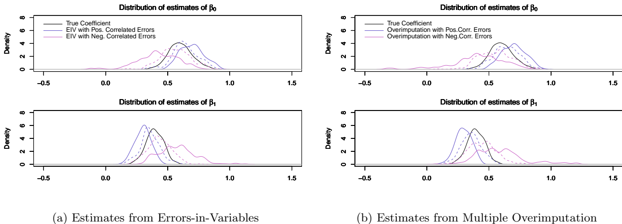
Figure 7: With data generated so that proxy variables have measurement error correlated with each other (so that new information is not available with measures) both EIV (left graphs) and MO (right graphs) gives biased estimates.
