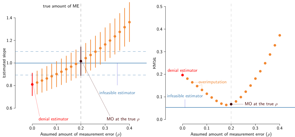
Figure 1: Simulation results with categorical latent and observed variables.
