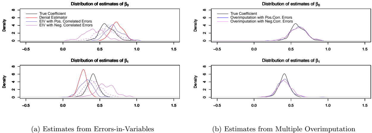
Figure 6: Here we show the estimates when the error in the instrument w_{i2} is correlated with the latent variable x_i . Positive (blue distributions) correlation leads to attenuated estimated effects in the errors-in-variables framework, and negative (violet) correlation exaggerates the effect, as shown in the left. The MO estimates show no bias.
