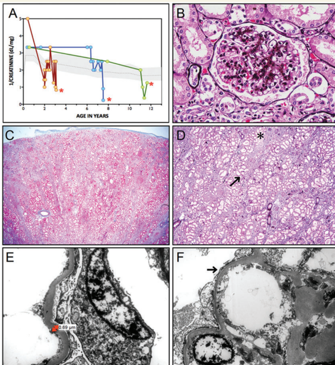
Figure 3 Kidney disease. (A) Variable onset of nephrosis is followed by progressive loss of glomerular function, shown as 1/\text{serum creatinine} (dl/mg), in three with NCS who died (red asterisks) from complications of renal failure at ages 3.5, 8, and 12 years. (B) Jones' stain reveals both global and segmental sclerosis of glomeruli. (C) 'Striped' fibrosis is seen throughout the kidney interstitium. (D) At higher magnification, linear tracks of fibrosis (arrow) correspond to adjacent tubular atrophy (asterisk). (E) Electron micrographs show a 3- to 4-fold thickening of the glomerular basement membrane (normal for age, 0.15\ \mu\text{m} ) accompanied by (F) effacement and microvillus transformation of podocyte foot processes (arrow).
