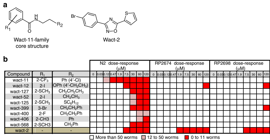
Figure 3 | Wact-11 and wact-12 resistant mutants are cross-resistant to all nine wact-11-family members. (a) The wact-11-family core structure and the structure of an unrelated molecule, wact-2, which was used as a negative control throughout this work. (b) Heat maps of the wact-11-family dose-response experiments with wild-type worms (N2 strain), as well as two mutant strains, RP2674 and RP2698, isolated as being resistant to wact-12 and wact-11, respectively. The dose-response experiments were carried out using a 96-well plate liquid-based assay (see Methods). White indicates that there were more than 50 worms in three out of four replicate wells. Pink indicates that there were between 12 and 50 worms in three out of four replicate wells. Red indicates that there were between 0 and 11 worms in three out of four replicate wells. In the case of ties, the higher number prevailed (for example, at a given concentration, if two wells had 55 worms, and the other two wells had 20 worms, the chemical would be scored as having more than 50 worms). The R 1 and R 2 groups are indicated for each wact-11-family member. Wact-2 is used here as a negative control.
