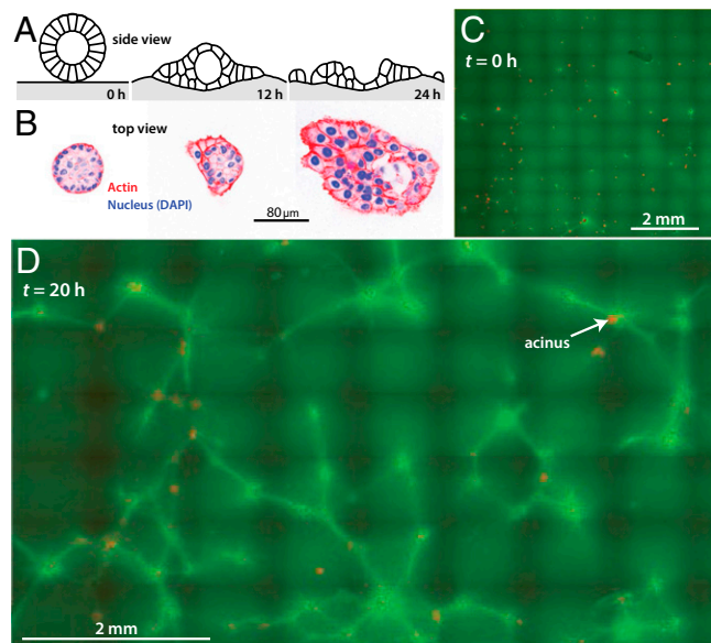
Fig. 1. Mechanical remodeling of collagen substrates by mammary acini. ( A ) Schematic of experiment. Acini are placed on collagen 1 gels and subsequent disorganization is quantified. ( B ) Acini allowed to settle on collagen gels gradually disorganize as shown by changes in acinar morphology (nuclei stained blue) and actin cytoskeleton (red). ( C ) Low-magnification overview of a system of \sim 200 acini (red) on collagen 1 (green). Initially, the collagen is uniformly distributed and the acini are intact. ( D ) System of \sim 200 acini after 20 h. Many acini (red) have disorganized into single cells (tiny red dots), which are scattering. The collagen has been extensively reorganized; the average green signal has dropped and bright green collagen lines run along geodesics between acini.
