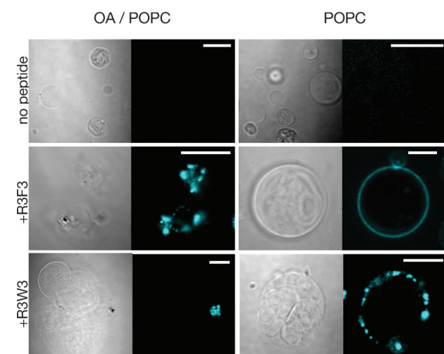
Figure 4. Microscopy of peptide-induced RNA–membrane association. Confocal images show RNA localization (5'-AlexaFluor647-labeled 15-mer, cyan) to the outside of oleic acid/POPC (90%/10%) and pure POPC membranes in the presence of R3F3 and R3W3 peptides. Control samples had no peptide added. For each image, the left panel shows the DIC image and the right panel shows AlexaFluor647 fluorescence. The scale bar is 20 \mu\text{m} .
