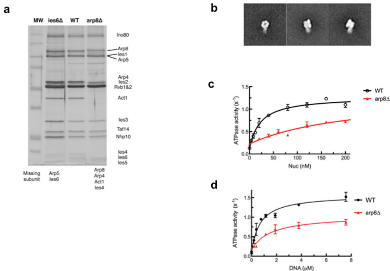
Figure 3. Functional analysis of the INO80-Carp 8 subcomplex (a) SDS-PAGE gel of INO80-C, INO80-Carp 8 and INO80-C ies6 subcomplexes. (b) Selected class averages of negatively stained INO80-Carp 8 subcomplex. Top view (left panel) and side view (middle and right panels). Side length of individual panels is 57.3 nm. (c) Nucleosome-stimulated ATPase activity of the INO80-Carp 8 subcomplex. (d) DNA-stimulated ATPase activity of the INO80-Carp 8 subcomplex. Each error bar represents the standard deviation from three independent experiments.
