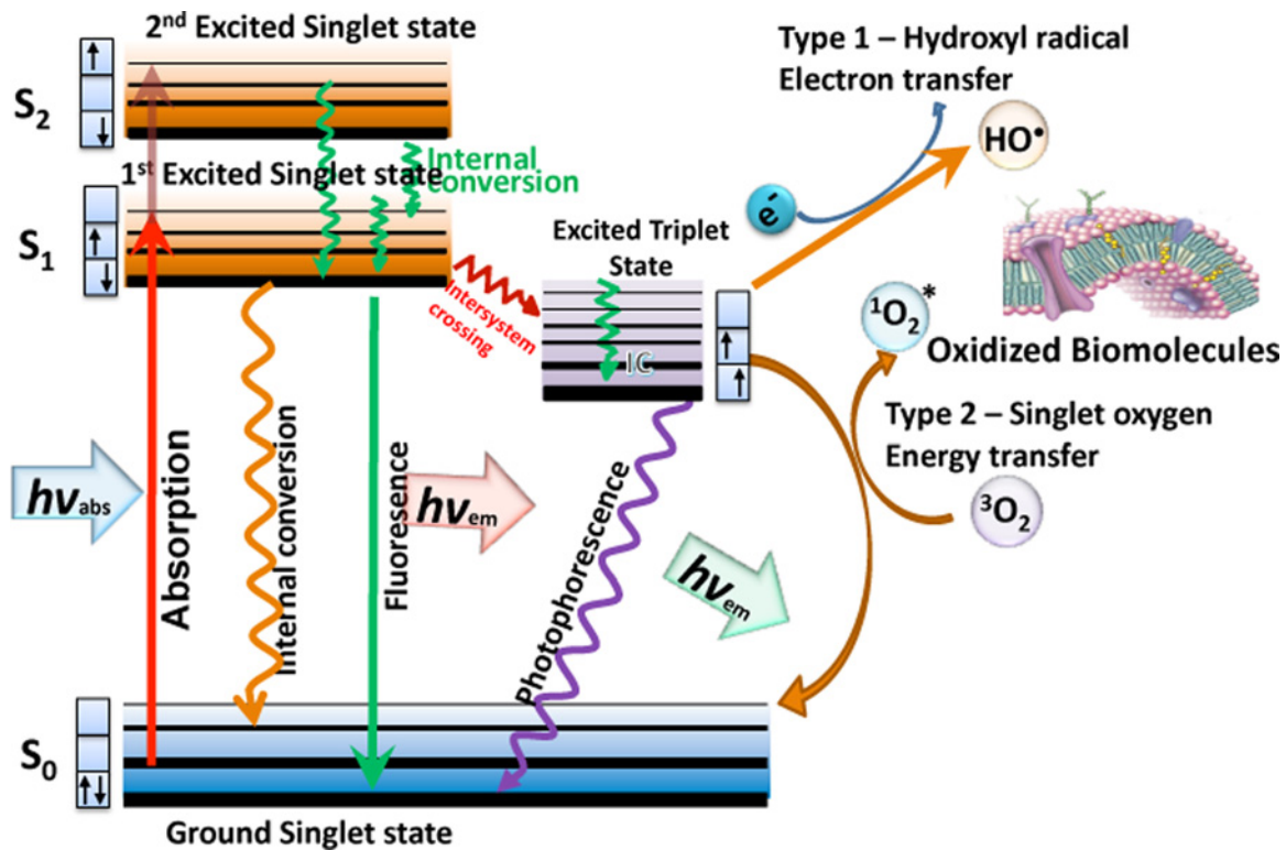
Figure 1 Jablonski diagram
