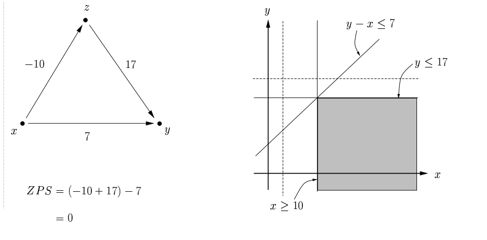
Figure 5.6: An xy -edge that is dominated by a path through zero
