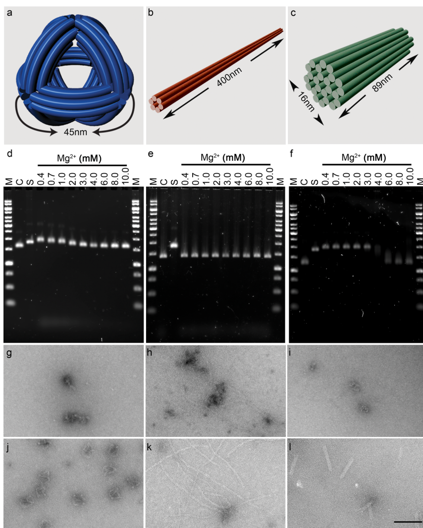
Figure 1. DNA nanostructure sensitivity to cation depletion in tissue culture medium. The three test nanostructures are (a) DNA nano-octahedron (DNO), (b) six-helix bundle nanotube (NT), and (c) 24-helix nanorod (NR). (d–f) Three nanostructures were incubated for 24 h at 37 °C in unmodified RPMI tissue culture medium containing 0.4 mM \text{Mg}^{2+} or adjusted to 0.7–10 mM \text{Mg}^{2+} , and the products were analyzed by agarose gel electrophoresis (AGE). In comparison to the control lanes of stable sample, migration of the DNO and NR is retarded after low \text{Mg}^{2+} incubation, indicative of denaturation, whereas no obvious difference in migration is observed with the NT. (g–i) Transmission electron microscopy images of nanostructures incubated in unmodified medium, showing varying levels of denaturation. (j–l) With RPMI medium adjusted to 6 mM \text{Mg}^{2+} , structural integrity is maintained in all three designs. M = molecular weight ladder, C = nanostructure in TE + 10 mM \text{Mg}^{2+} , S = M13 scaffold. Scale bar = 100 nm.
