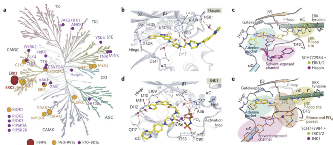
Figure 3. Selectivity and off-target binding modes of SCH772984
