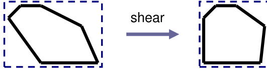
Figure 3: The convex hull (black) is surrounded by the minimum area rectangle aligned with the bottom edge. Since both left and right extents of non-bottom edge points are to the left of their respective bottom edge extents, we can apply an affine shear to shift the points right so that the leftmost non-bottom edge point aligns with the leftmost edge point. After shearing, fewer samples are wasted.
